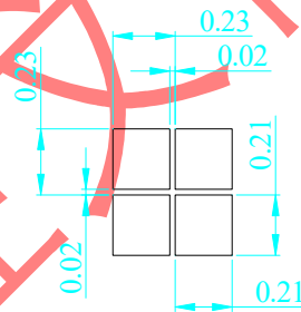
Detail Dots size Scale 10/1
